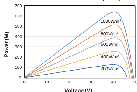
P-V CURVES OF PV MODULE (640W)
