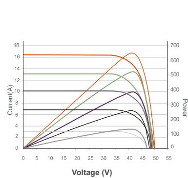
Current voltage and power voltage (640W)
