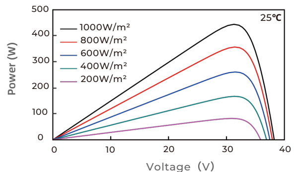
P-V Characteristics At Different Irradiations
