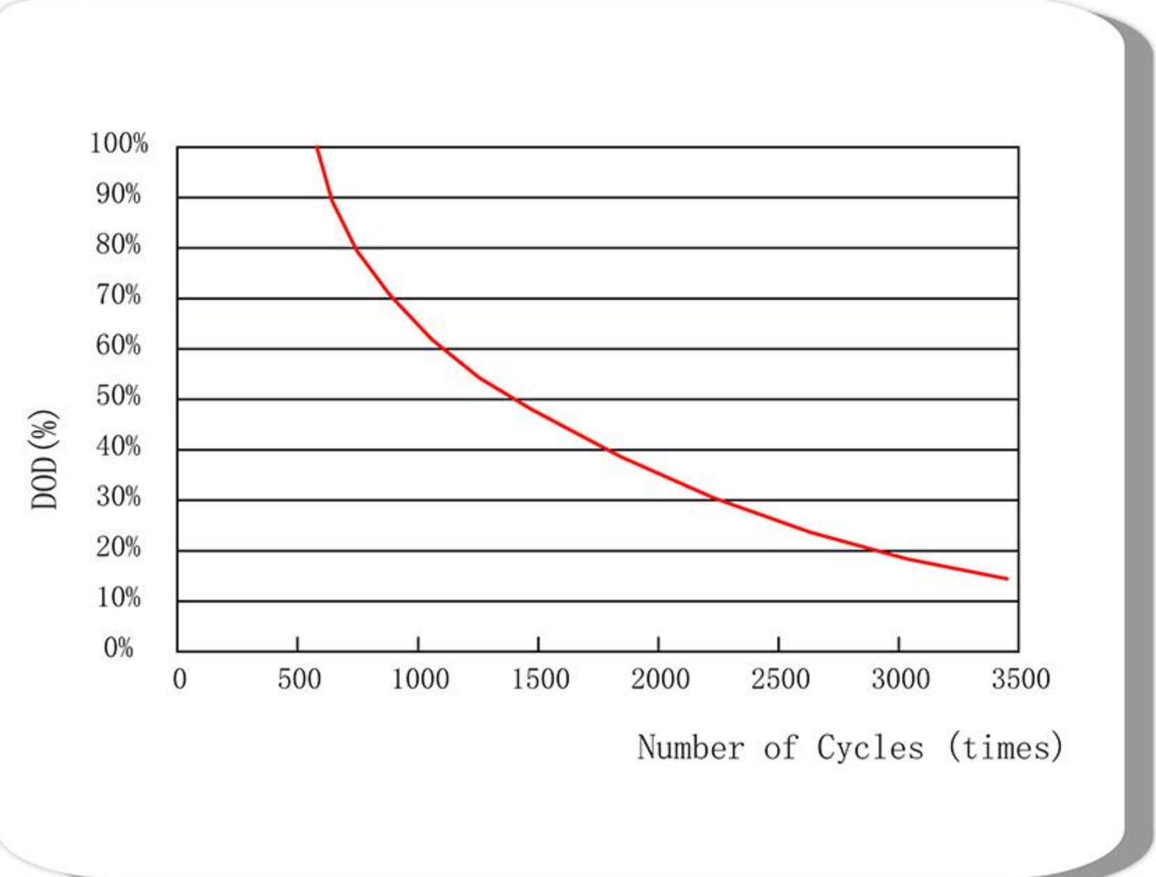
Cycle Service Life (25°C/77°F)
